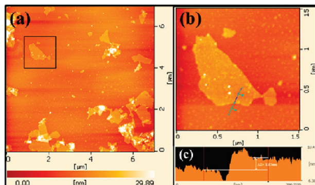
Figure 1. (a) Tapping-mode AFM image of graphene oxide. (b) Enlargement of a piece of graphene oxide. (c) Height profile through the line shown in (b).
