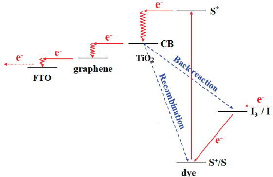
Scheme 2. Operational principle of the device: the introduced 2D graphene bridges perform as an electron acceptor and transfer the electrons quickly. Hence, the recombination and back reaction are suppressed.
