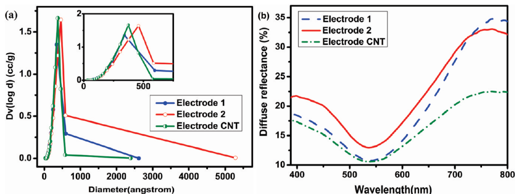
Figure 6. (a) BJH pore size distributions calculated from N 2 desorption isotherms, and (b) measured diffuse reflectance of sensitized anodes.
